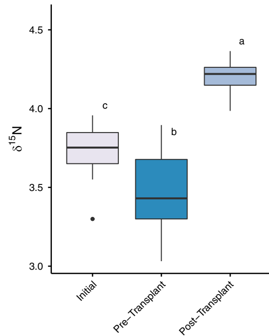
Fig. 3 Box and whisker plots of the median \delta^{15}\text{N} in Sargassum mangarevense tissue across three treatments from a short-term transplant experiment, showing the third quartile (Q3) and first quartile (Q1) range of the data, the whiskers (95% quartile) and data outliers. Connecting letters indicate significant differences between treatments. Stable isotopic signatures were measured in subset samples of the same specimens that were collected from a low-nutrient reef (initial), placed in laboratory aquaria to deplete internal nutrient stores for \sim 7 days (pre-transplant), before they were deployed on the bleached reef for 3 weeks (post-transplant) ( n = 10 )
