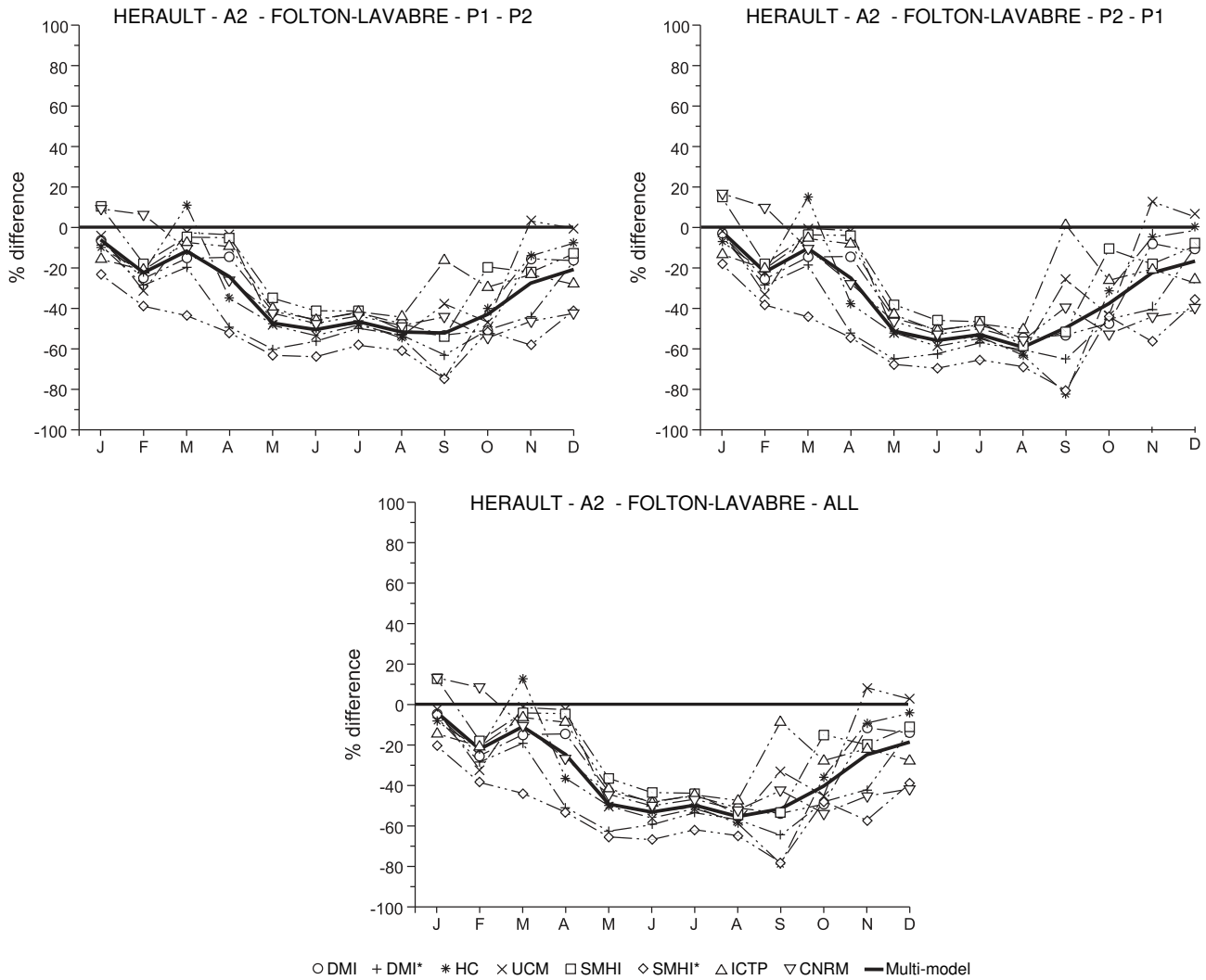
Fig. 10. Changes (in%) in the mean monthly discharge simulated by the GR2M model calibrated on different periods according to the full split-sample test of Klemesš (1986) between the periods 1961–1990 and 2071–2100 for the Hérault River for the A2 scenario. The RCMs marked with an asterisk were forced by the outputs of the GCM ECHAM4/OPYC3.
