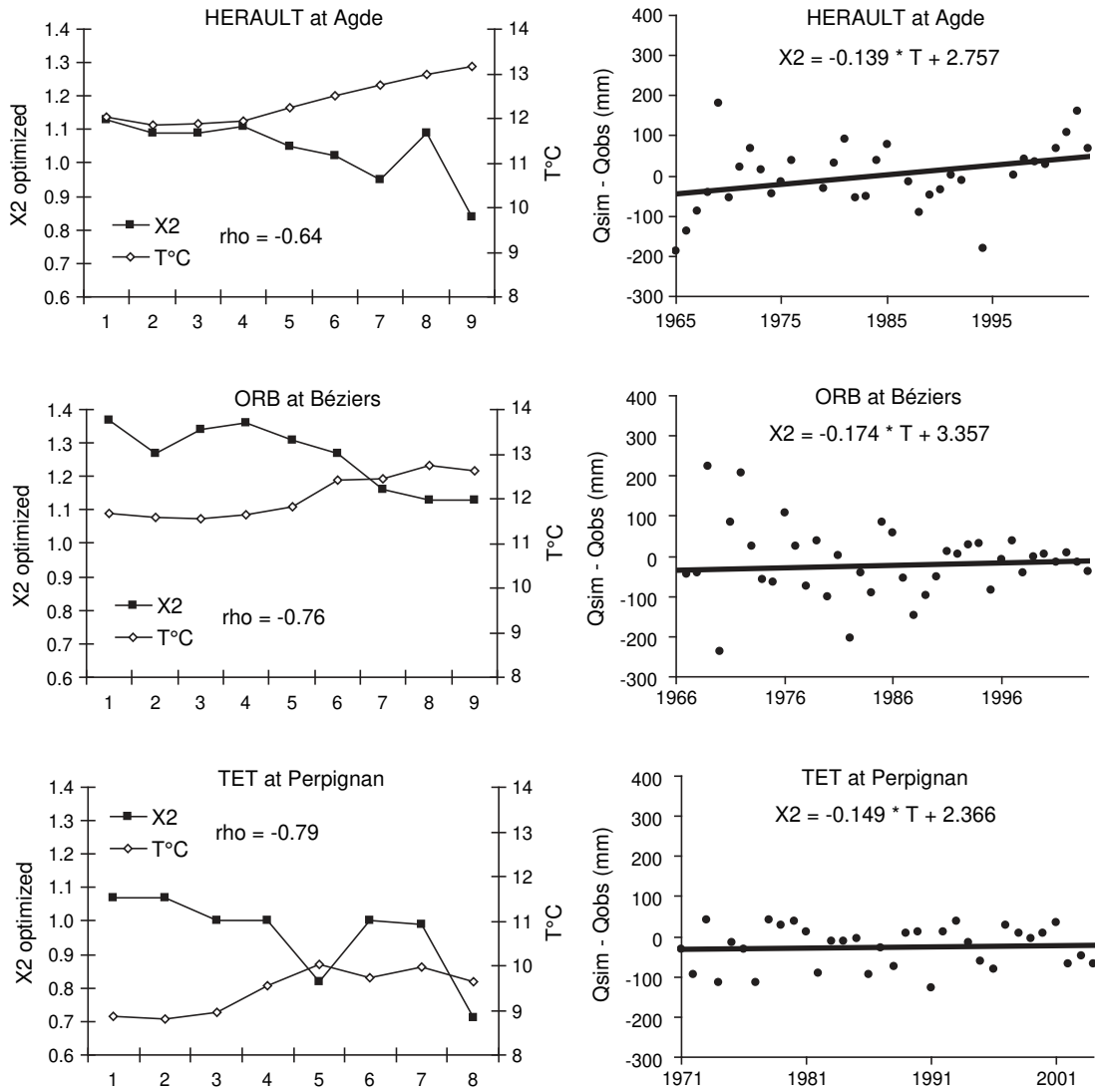
Fig. 11. Correction of the GR2M model drifts for the Héroult, Orb and Têt rivers. Left panels: Evolution of the optimized X_2 parameter value and mean annual temperature over the successive calibration periods. The rho values are the Spearman's correlation coefficients calculated between both time-series. Right panels: Time-series of differences (in mm) between the mean annual discharge simulated by the GR2M model with temperature-varying X_2 values and observations over the period 1965–2004.
