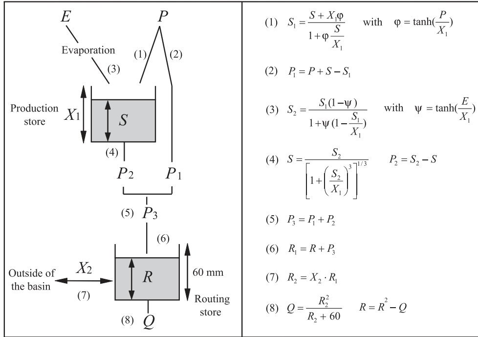
Fig. 4. Structure of the GR2M model (adapted from Mouelhi et al., 2006).
