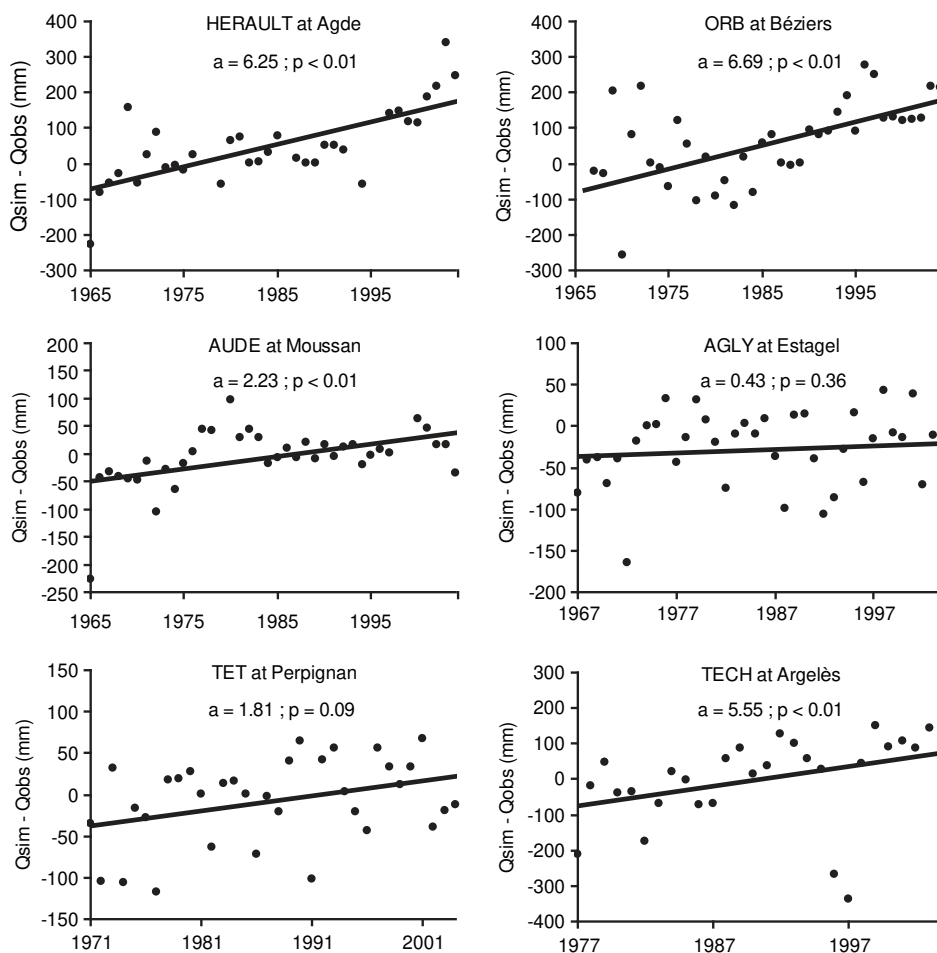
Fig. 5. Time-series of differences (in mm) between the mean annual discharge simulated by the GR2M model calibrated over the 1965–1984 period (reference parameter set) and observations over the period 1965–2004. Slopes of the trends ( a ) as well as significance of the trends according to the Mann–Kendall test ( p ) are also shown.
