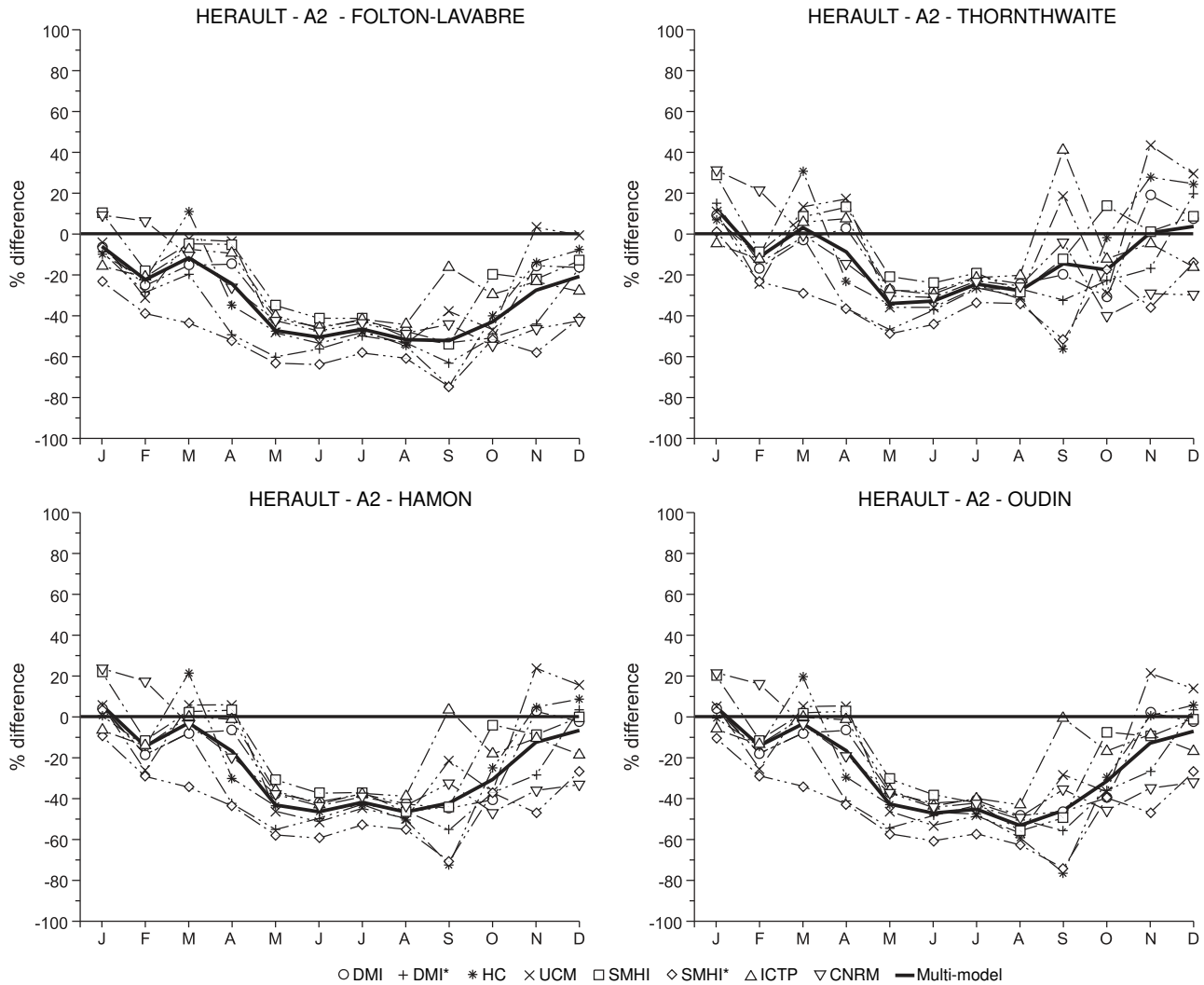
Fig. 9. Changes (in%) in the mean monthly discharge simulated by the GR2M model calibrated over the 1965–1984 period (reference parameter set) between the periods 1961–1990 and 2071–2100 for the Hérault River with different PE formulations for the A2 scenario. The RCMs marked with an asterisk were forced by the outputs of the GCM ECHAM4/OPYC3.
