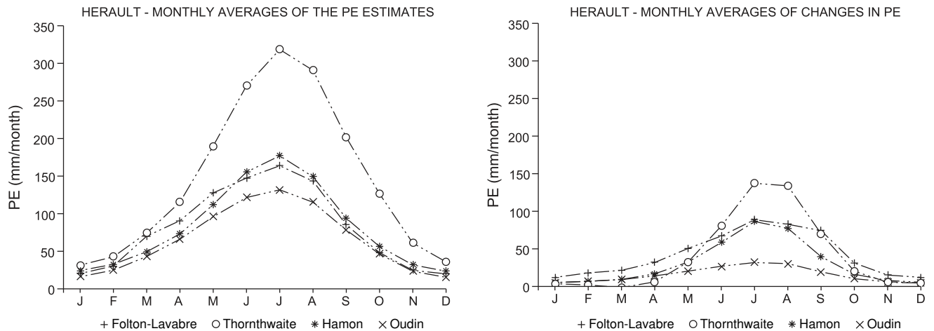
Fig. 8. Mean monthly PE over the period 1965–2004 and changes for the period 2071–2100. Left panel. monthly averages of the PE estimates over the period 1965–2004 for the Hérault River Basin with different PE formulations for the A2 scenario. Right panel: changes (in mm/month) between the periods 1961–1990 and 2071–2100 for the Hérault River Basin with different PE formulations for the A2 scenario.
