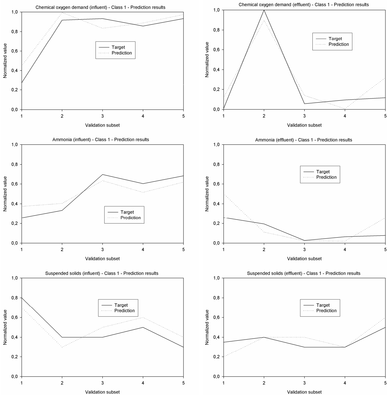
Fig. 7. Estimation results for COD, NH 4 and SS (influent and effluent)
