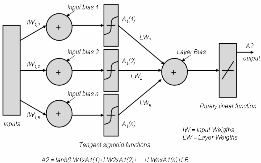
Fig. 3. MLP neural network structure
