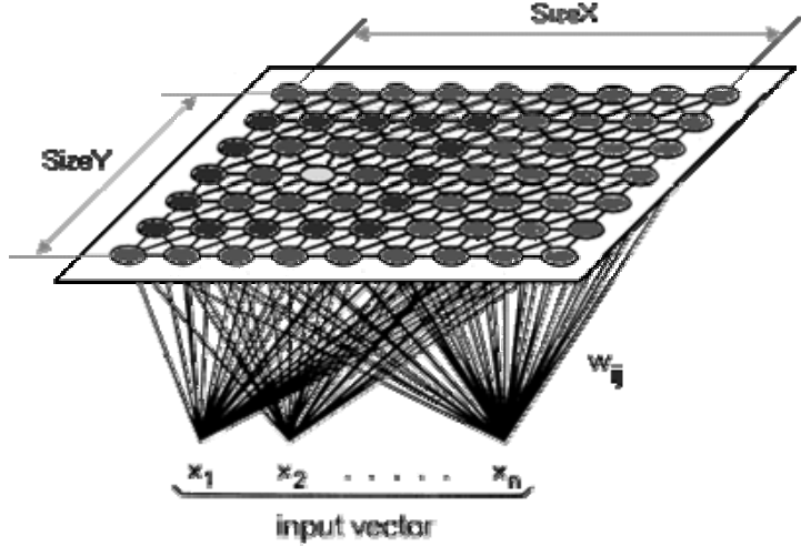
Fig. 2. Kohonen network structure
